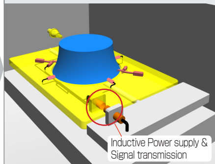
Turning the jig while machining
